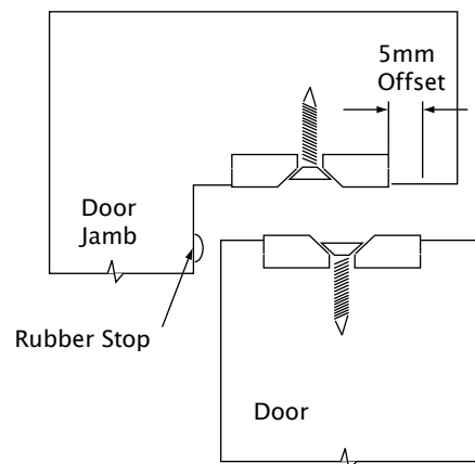
Installation Diagram
